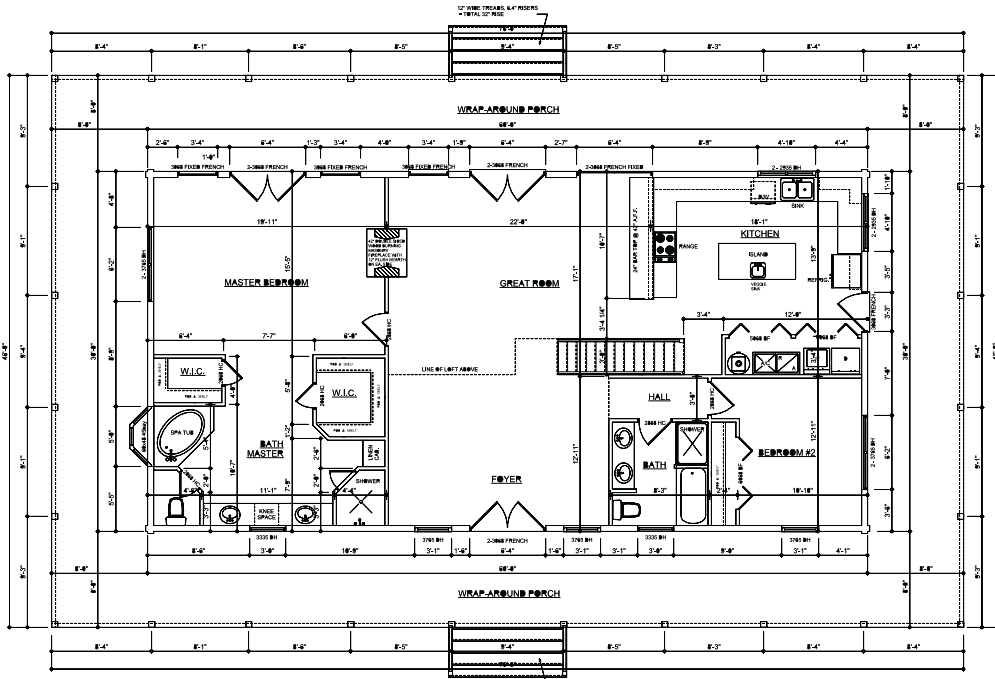
FLOOR PLAN SCALE: 1/8" = 1'-0" NOTE: ALL CEILING HEIGHTS SHALL BE 8'-0" UNLESS OTHERWISE NOTED
