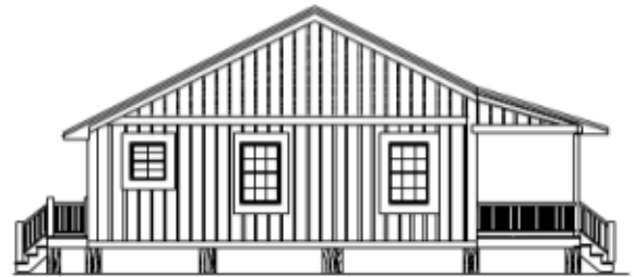
LEFT ELEVATION
